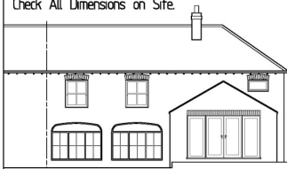
East Elevation. (1:100)
