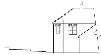
West Elevation. (1:100)
